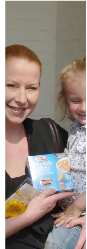
Elternsampling
